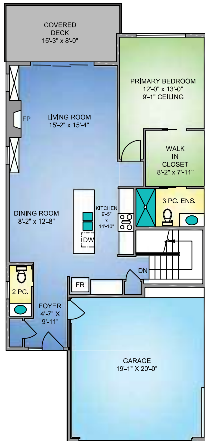
MAIN FLOOR 1058 SQ. FT. 9'-1" CEILING HEIGHT
