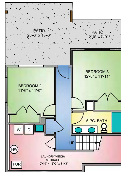
LOWER FLOOR 793 SQ. FT. 8'-0" CEILING
