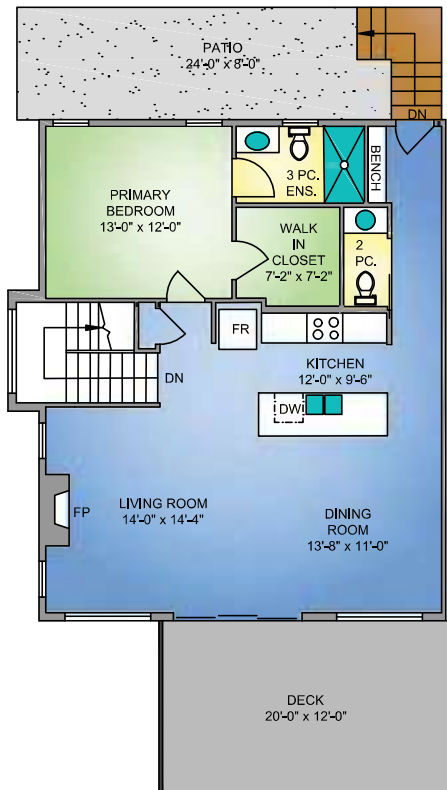
MAIN FLOOR 1009 SQ. FT. 9'-1" CEILING HEIGHT
