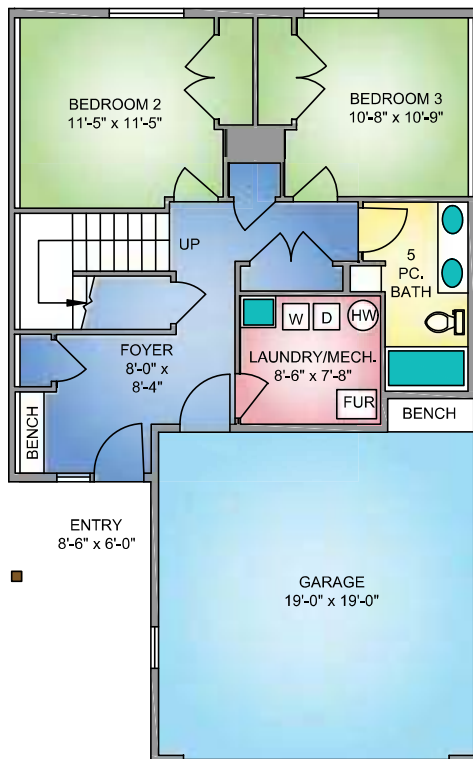
LOWER FLOOR 751 SQ. FT. 9'-0" CEILING
