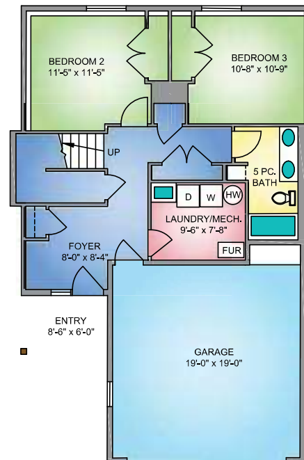
LOWER FLOOR 768 SQ. FT. 8'-0" CEILING
