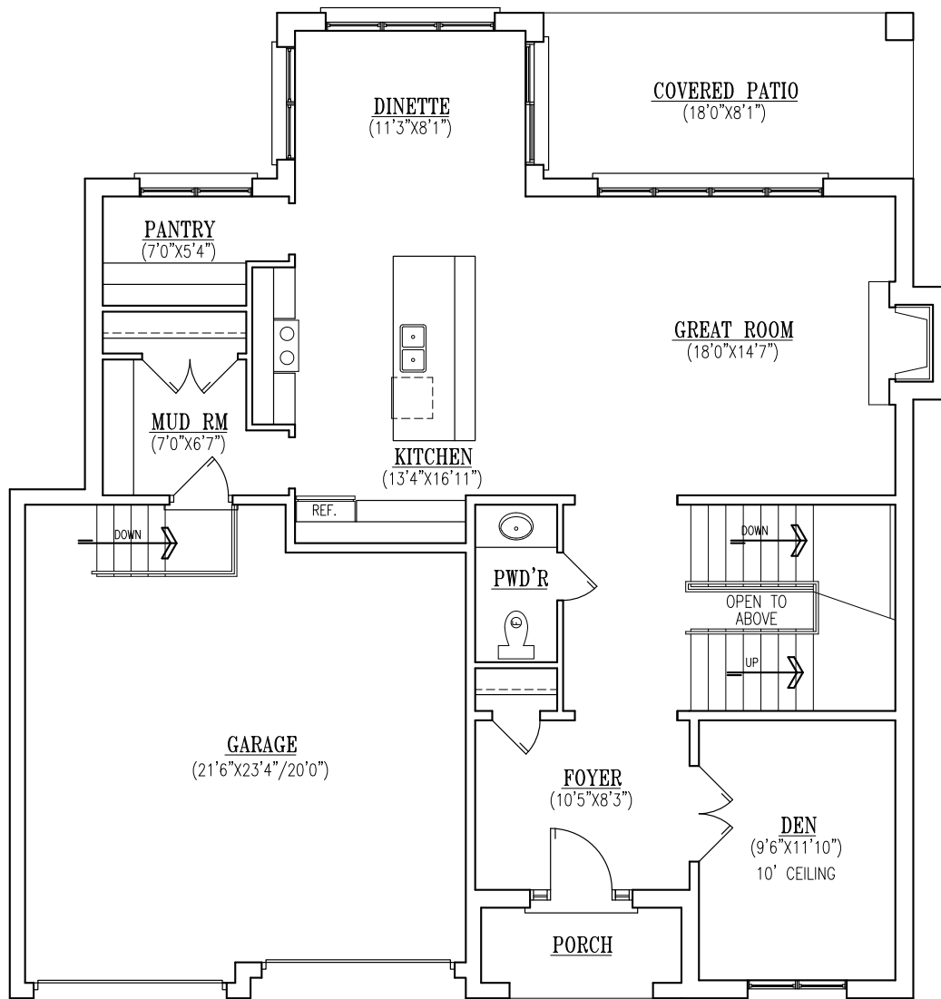
MAIN FLOOR PLAN PART 7 LONGWORTH ROAD
