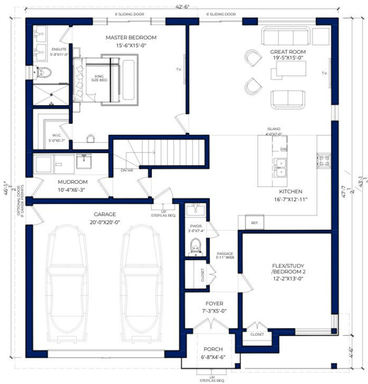
FIRST FLOOR AREA = 1,422 SQ FT
