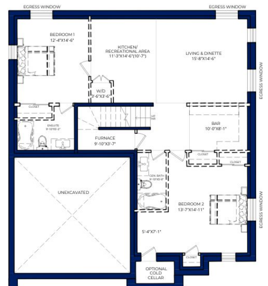
OPTIONAL FINISHED BASEMENT FLOOR AREA = 1,437 SQ FT
