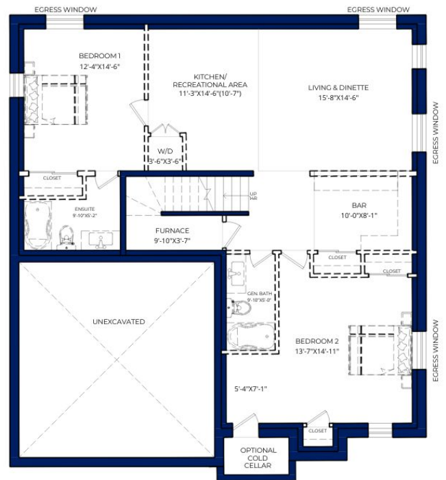
OPTIONAL FINISHED BASEMENT FLOOR AREA = 1,437 SQ FT
