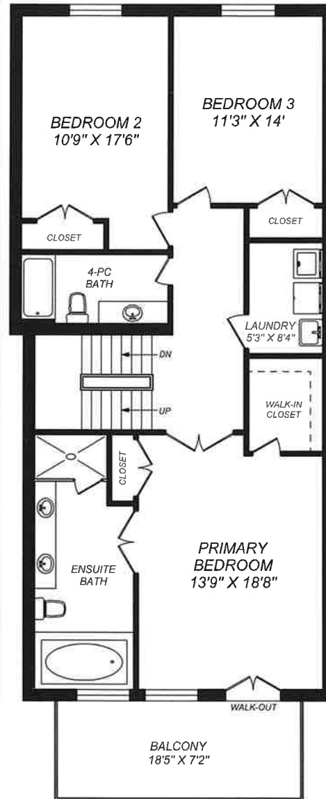
SECOND FLOOR 1213 SQUARE FEET (CEILING HEIGHT : 9'-0")
