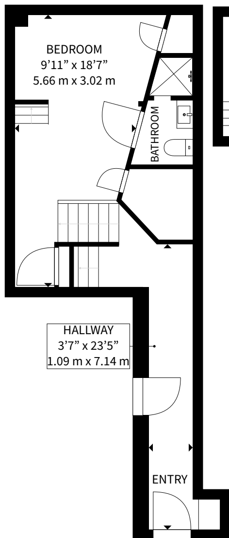
FLOOR 1
