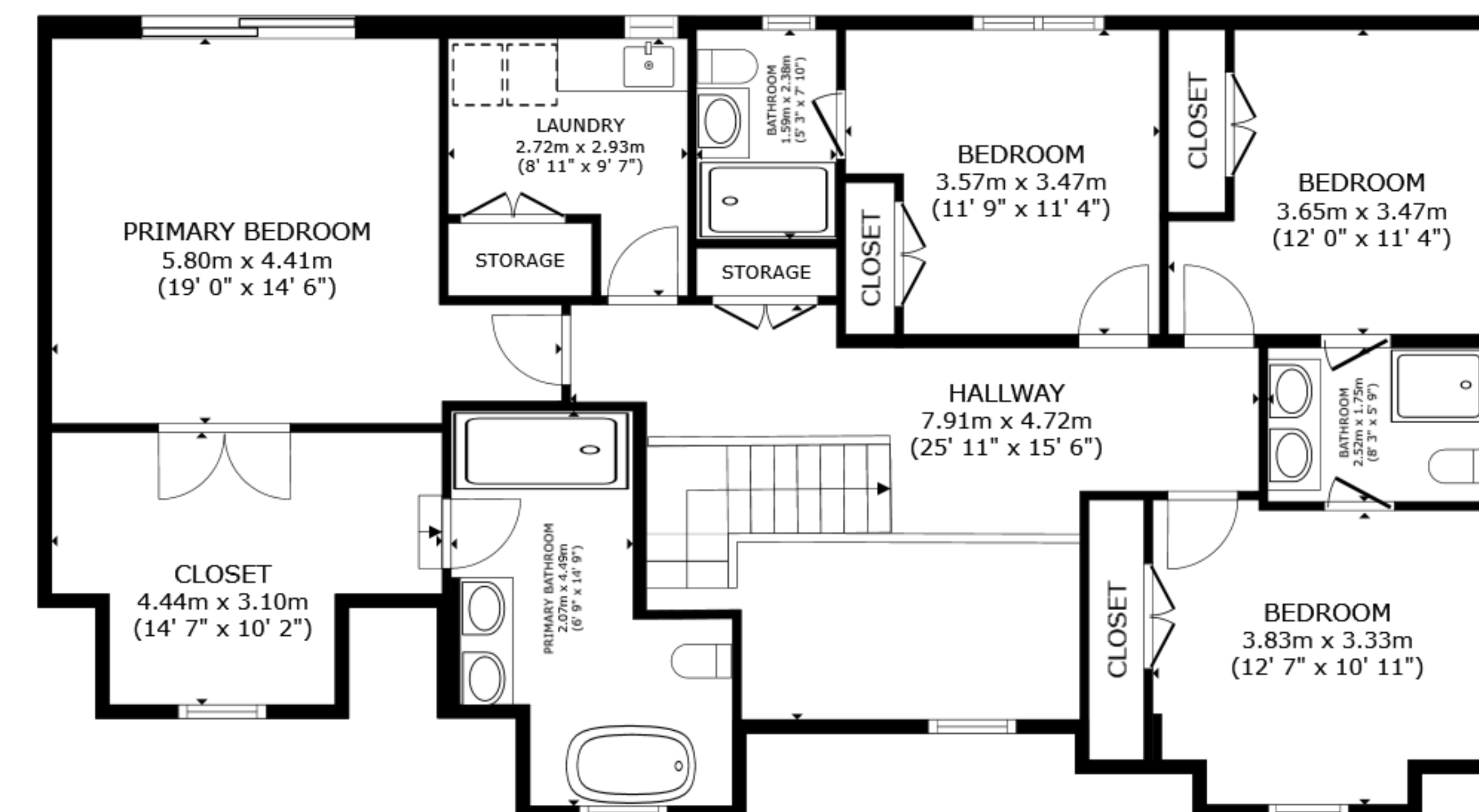
FLOOR 3
