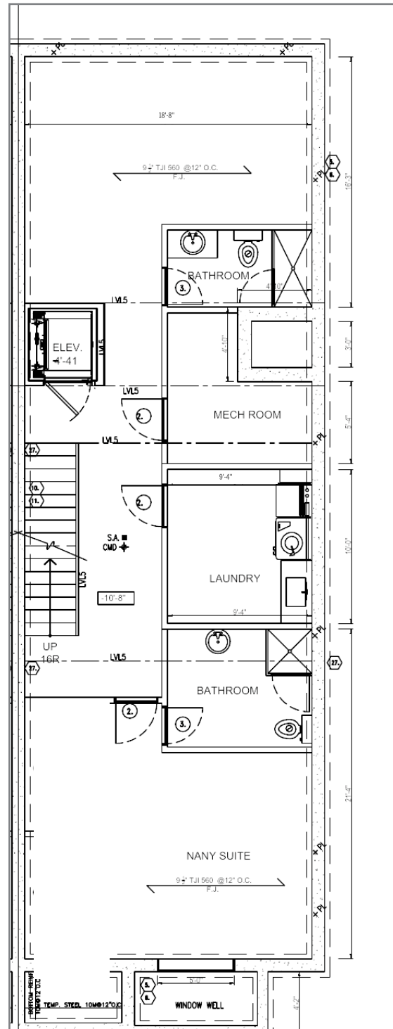
LOWER LEVEL
