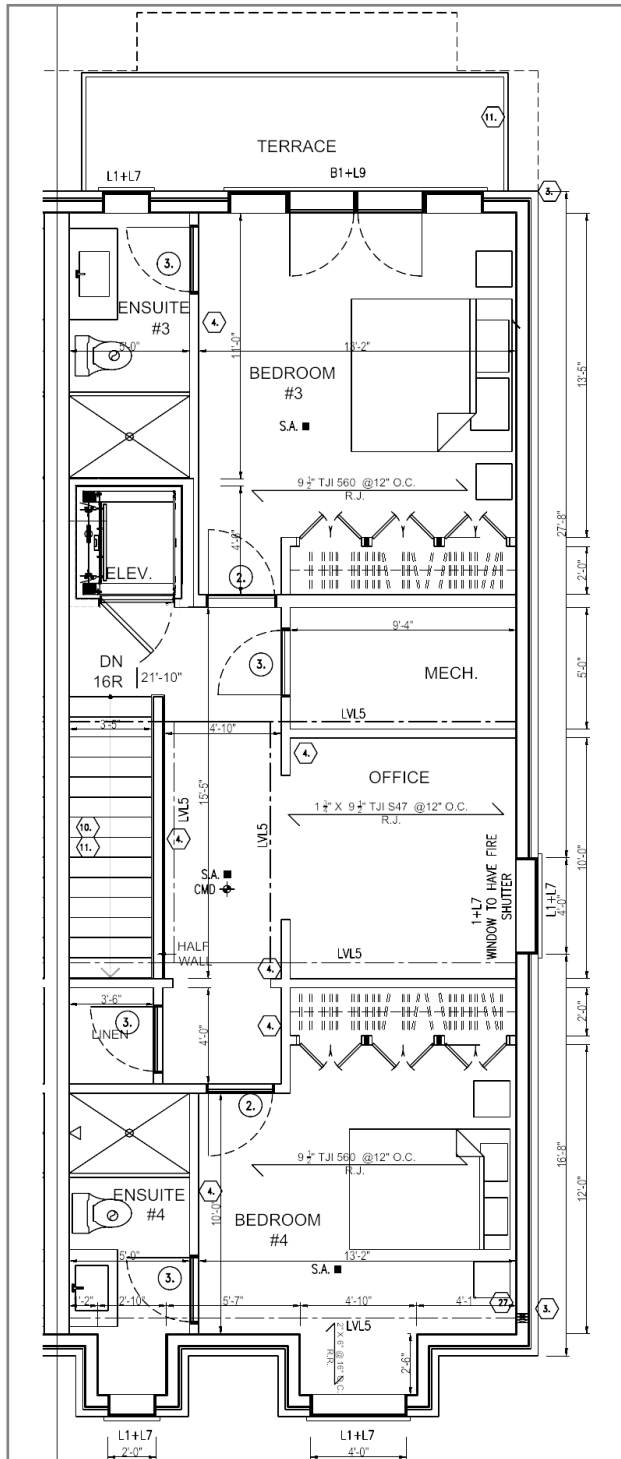
THIRD FLOOR
