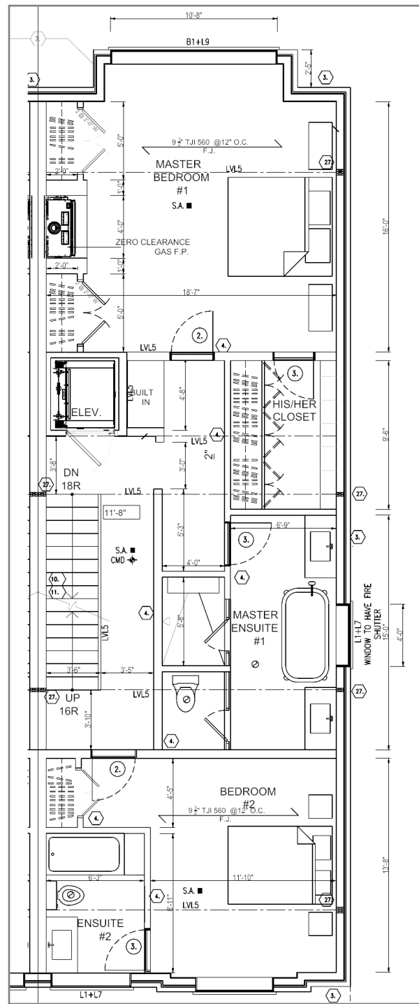
SECOND FLOOR
