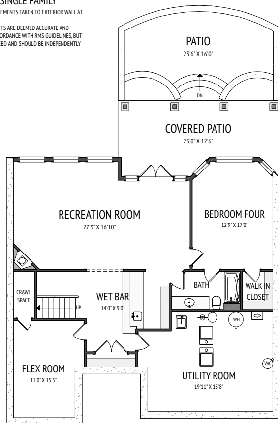
BASEMENT 1669.66 SQ.FT.
