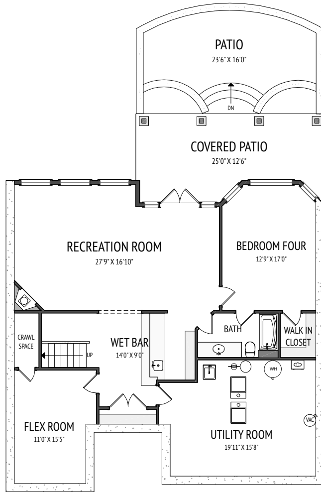
BASEMENT 1669.66 SQ.FT.
