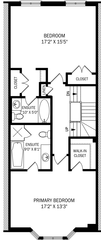
SECOND FLOOR - 845 SQUARE FEET
