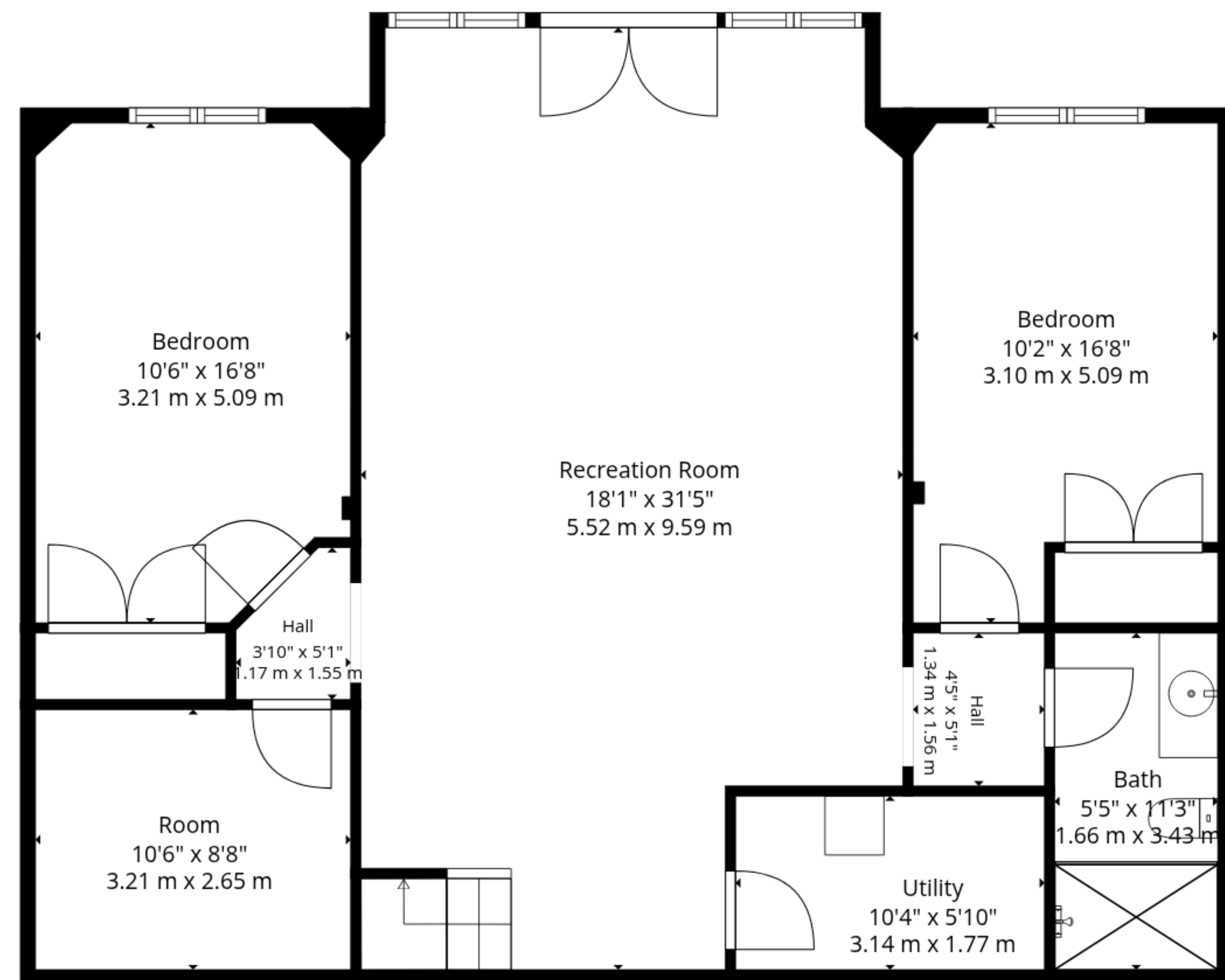
Basement 1
