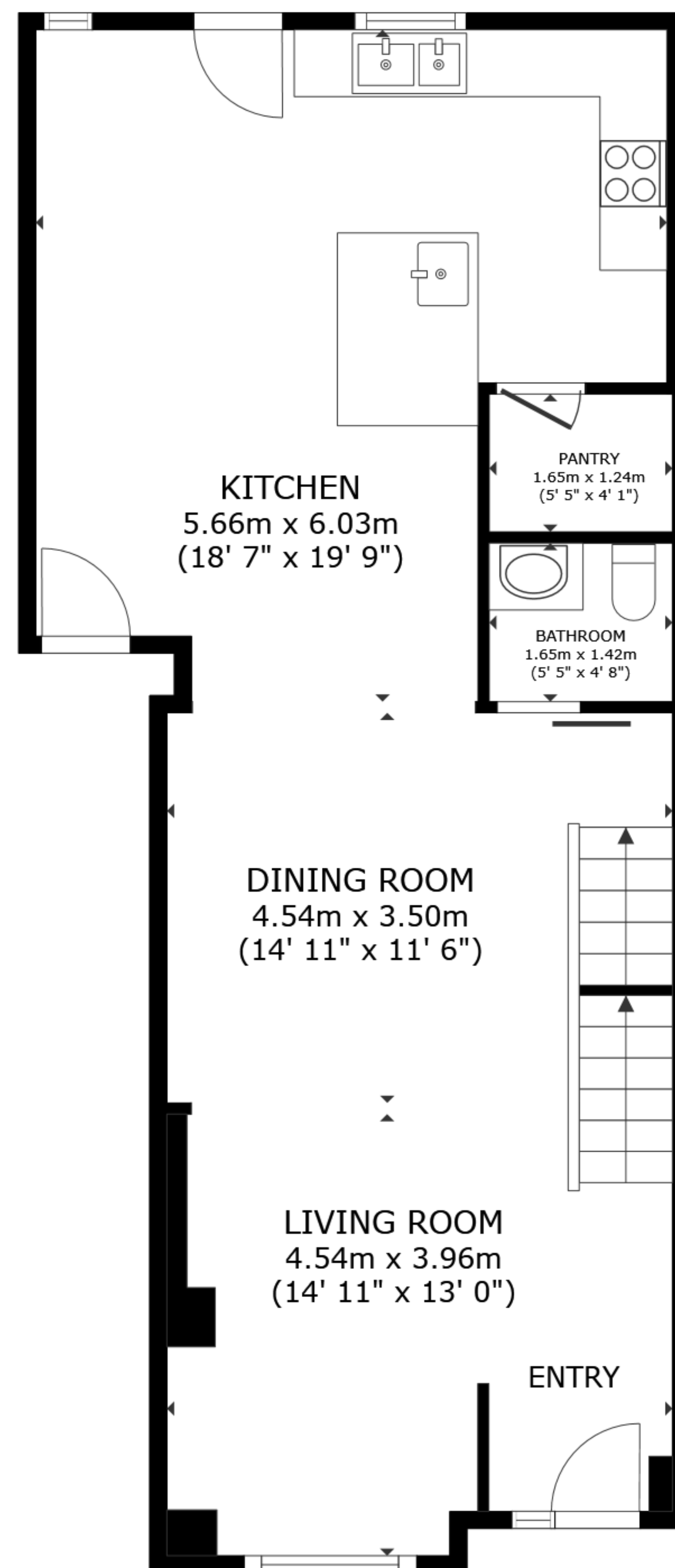
MAIN FLOOR
