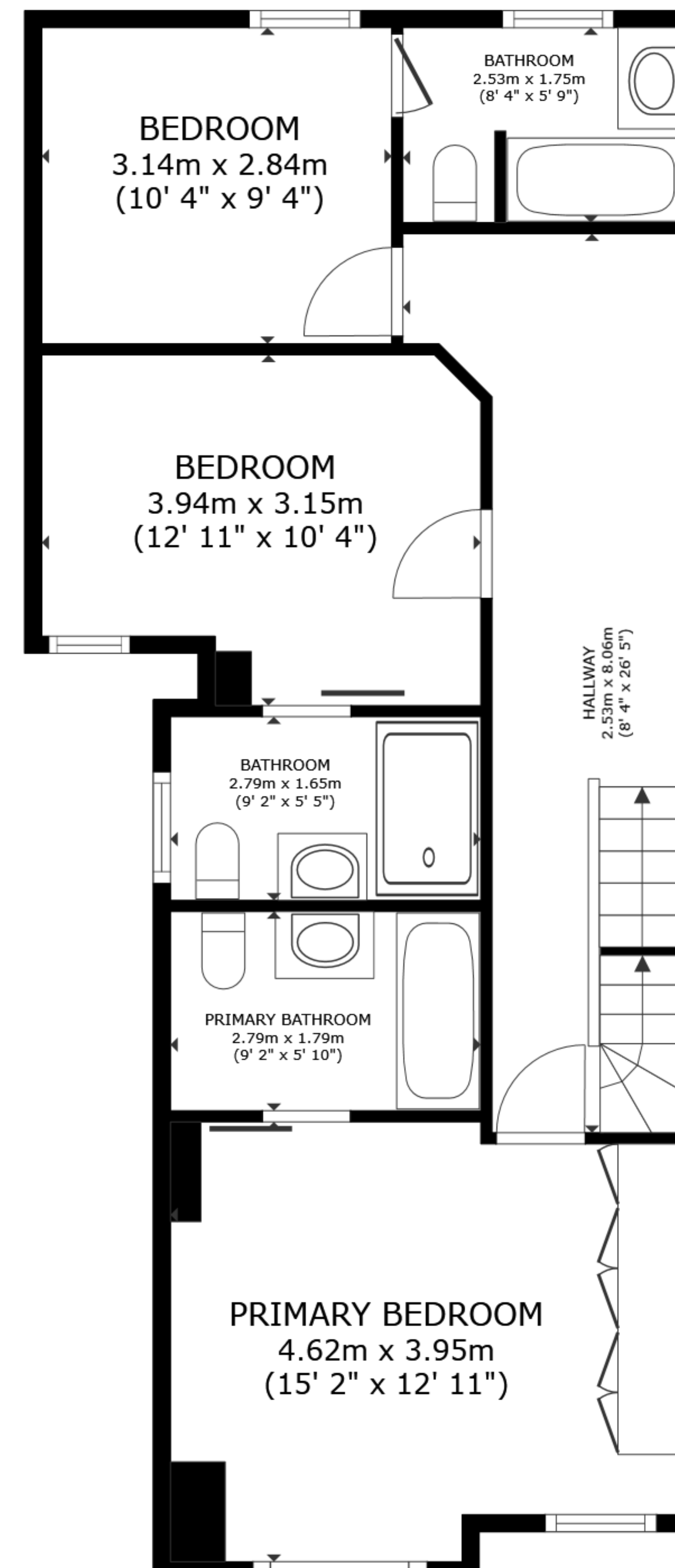
SECOND FLOOR
