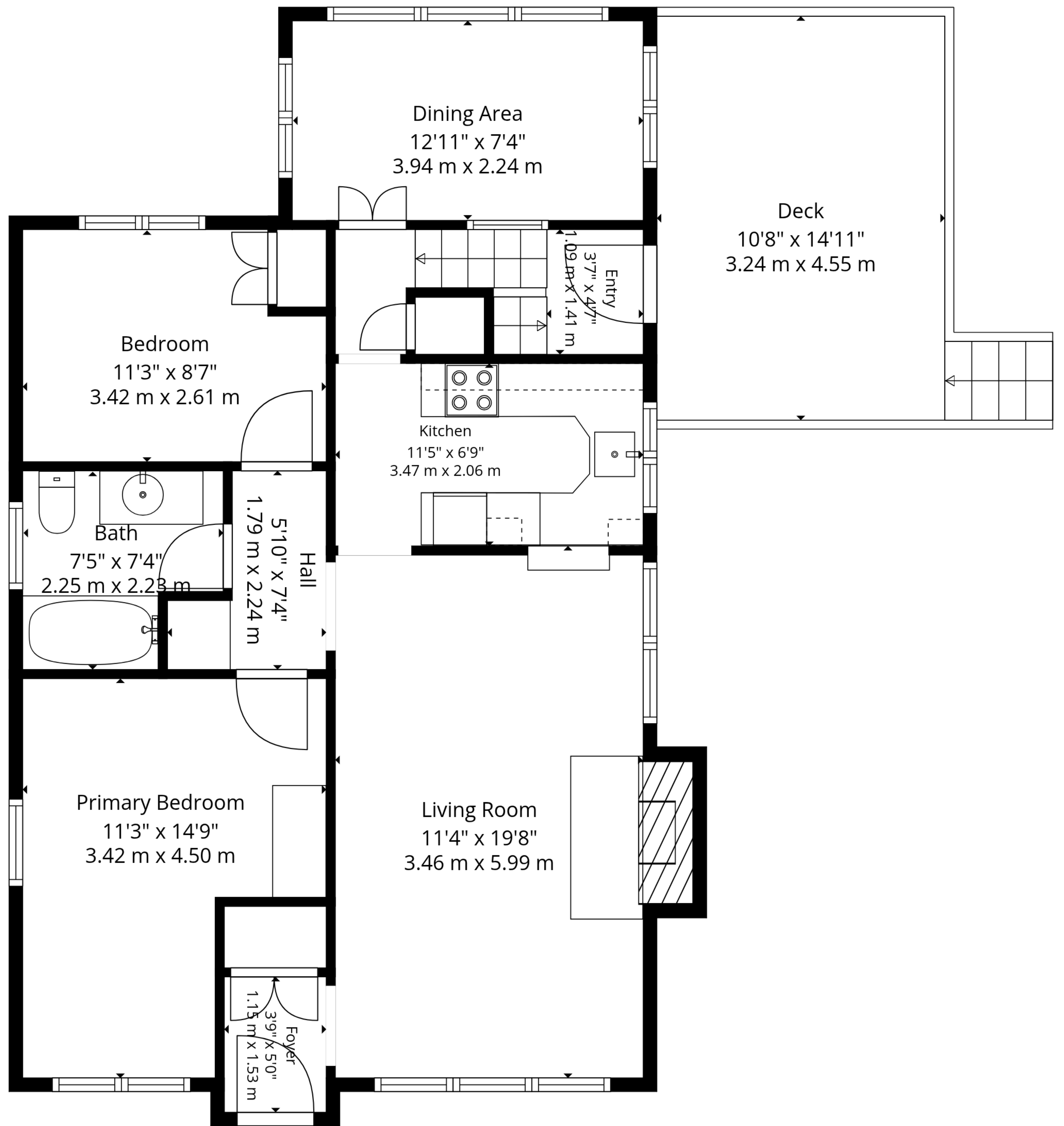
1st Floor
